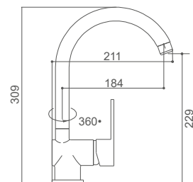
ORD0235C Monomando para cocina vertical Kitchen mixer Mitigeur de cuisine vertical
