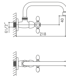
SAF6007C Monobloc para cocina pared Wall Kitchen mixer Melangeur de cuisine
