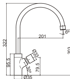
T03 Grifo vertical Temporizado Time delay vertical tap Robinet temporisé
