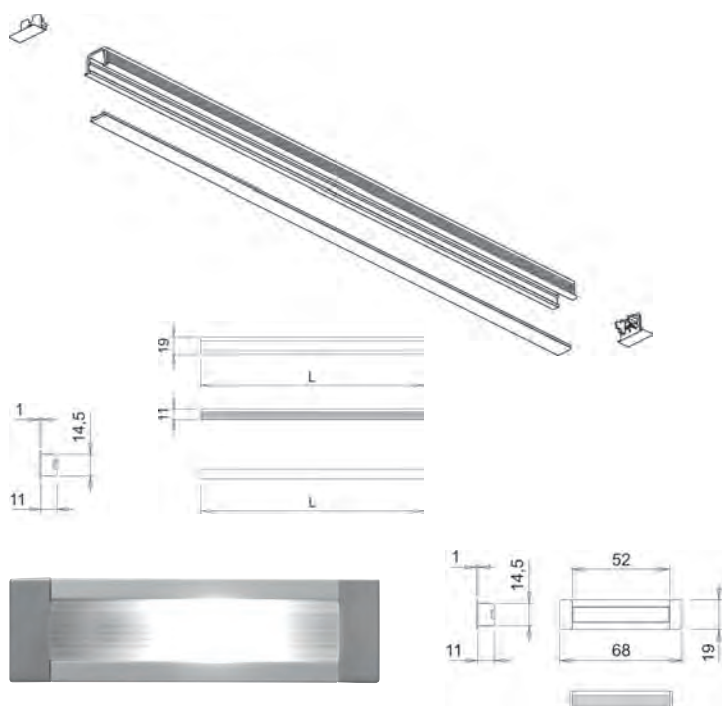
Sensor TOUCH LED DIVA
