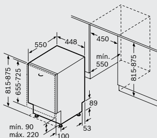
SMV88TX36E, SMV68MX03E, SMV46MX03E SMV46IX03E, SMV51E40EU, SMV41D10EU Dimensiones en mm
