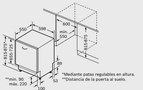
SMV88TX36E, SMV68MX03E, SMV46MX03E SMV46IX03E, SMV51E40EU, SMV41D10EU Dimensiones en mm
